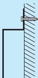
Screws through an up-fold, ideal for places where space is limited
