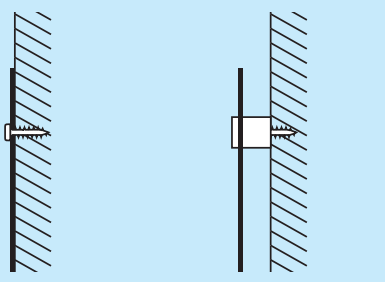
Pozi Head Screws or screws with Screw Caps
