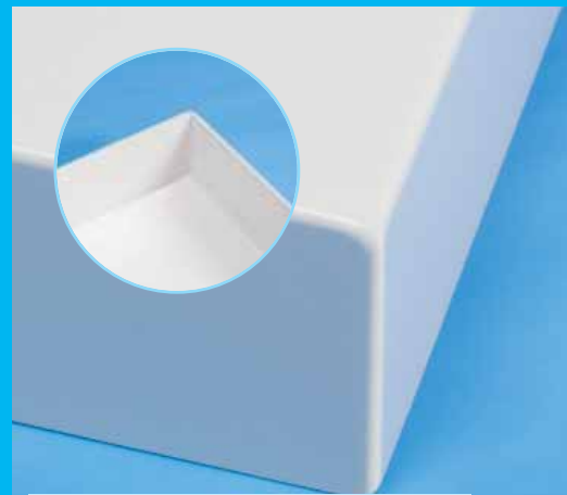
Aluminium tray with welded and smoothly dressed corners
