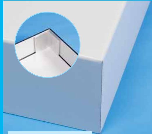
Composite tray with 'mitred' corners
